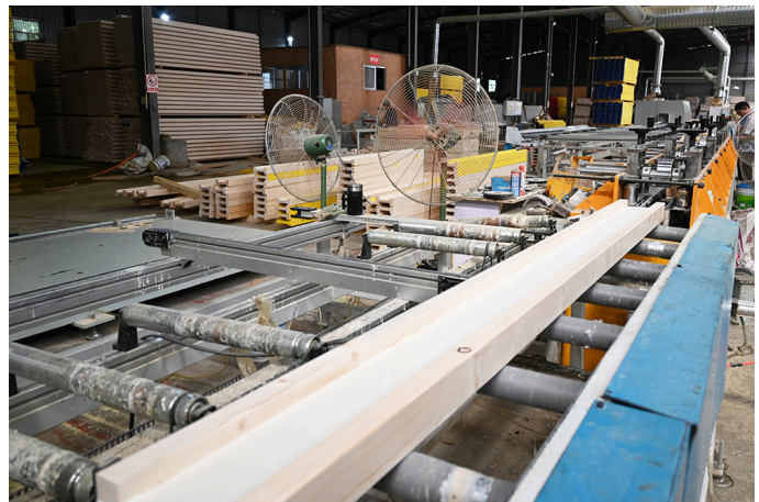
H20 Beam Production Line
