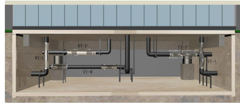
Flexible pipeline
