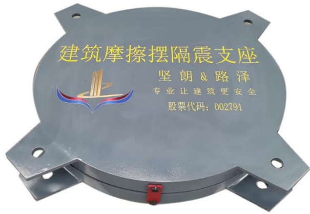
Friction Pendulum Bearings(FPB)
