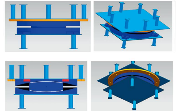
Separation-Resistant Friction Pendulum Bearings
