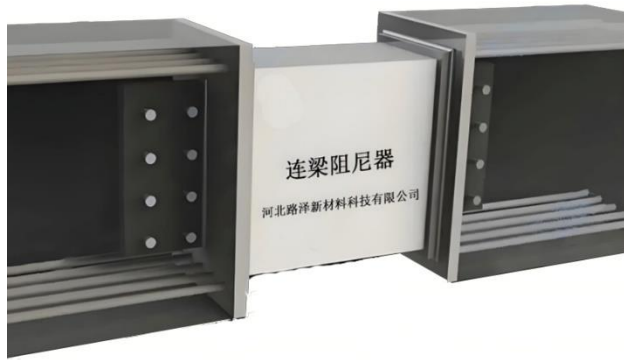
Coupling Beam Damper(CBD);
