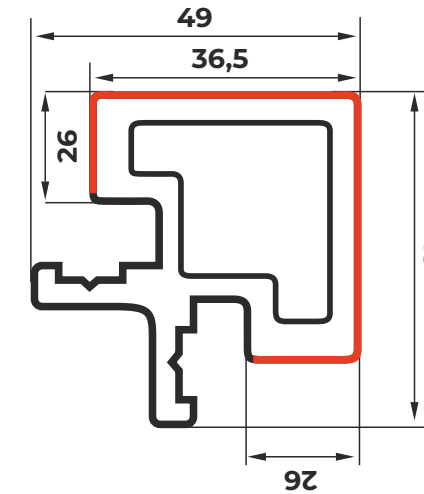
WPC Cross-sectional Diagram: 49mm*49mm
