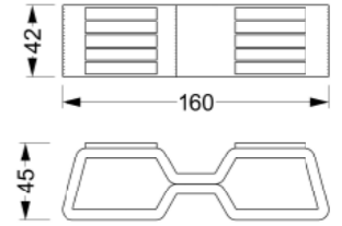
3D Safe Bank / 3D Safe Bench Kod / Code : 408 11 000000 058 Ağırlık / Weight : 250 kg
